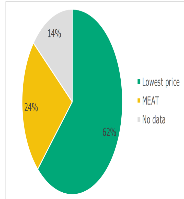
Figure II: Award criteria in PPM in the study countries, 2008-2021
